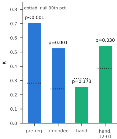
b Numeric herding \kappa
