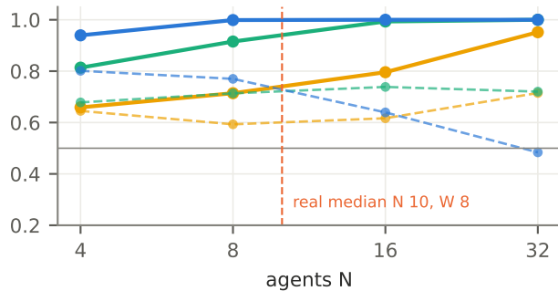
AUC, regrouping vs stationary
