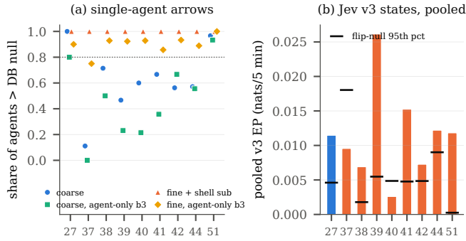
Second figure. (a) Share of agents beating the detailed-balance null per period. Fine classes with shell sub-classes (triangles) are irreversible for everyone and stay so with the scaffold removed (diamonds); the coarse arrow (dots) mostly does not survive removal (squares). (b) Pooled Jev v3 entropy production per 5-min transition (bars) and the block-flip null's 95th percentile: regime I (#27, blue) is not above regime III.
