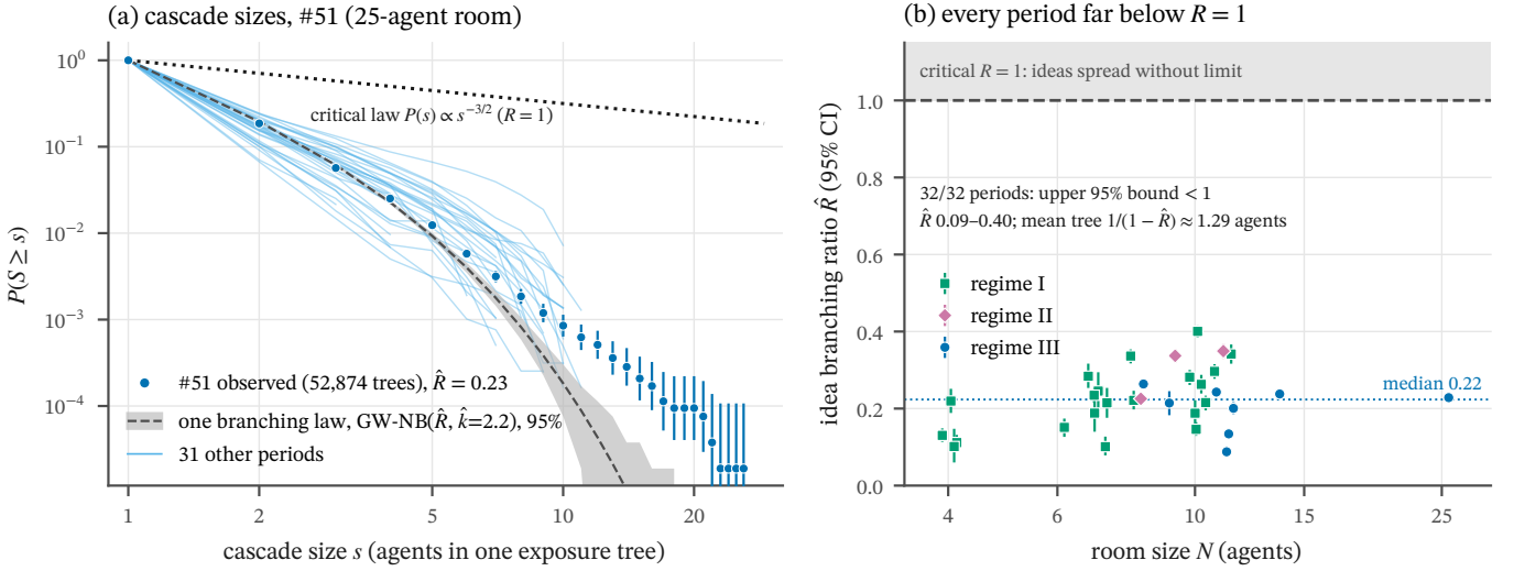
FIG. 14. Idea cascades are subcritical in every goal period (model 03, H34; round-1b data). (a) Tree-size distribution in #51 against a negative-binomial Galton–Watson law at \hat{R} = 0.23 and against the critical law P(s) \propto s^{-3/2} ( R = 1 ); thin lines are the other 31 periods. (b) \hat{R} with 95% CI for the 32 non-reserved periods against room size. Look at panel (b): every upper bound sits below 1. Round 2 adds that the heavy tail is a spread of R across ideas.
