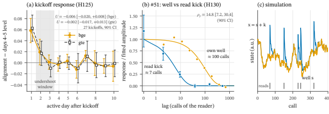
FIG. 4. A fast read kick on a slow, overdamped well (model 16). (a) After a goal kickoff, alignment with the kickoff (relative to its level on days 4–5) overshoots on day 1 and settles by day 3; nothing dips in the gray undershoot window ( U = -0.006 [-0.020, +0.008] (bge), 27 kickoffs, 90% CI; H125). (b) In #51 the memory of an agent for its own content (orange) decays over about 100 of its calls, while the pull of a read (blue) decays in about 7 (H130). We divide each series by its fitted amplitude; thin lines are e^{-\gamma n} . (c) Simulation: state x = slow well s + short kicks at reads (ticks). Look at the gap between the two curves in (b): one rate cannot describe both.
