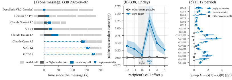
FIG. 2. A message acts at the read-out call of the recipient (model 02, H08). (a) One G38 message: room-mates with a call in flight read it 7–24s later at their next call; agents in long gaps read it 130–169s later and reply at that call. (b, c) The excess chance that a call names the sender jumps at the read-out call ( o = 1 ) and not at the call in flight ( o = 0 ), in G38 and in 17 periods outside the reserved data. Look at the step between o = 0 and o = 1 , and at the flat other-room placebo.
