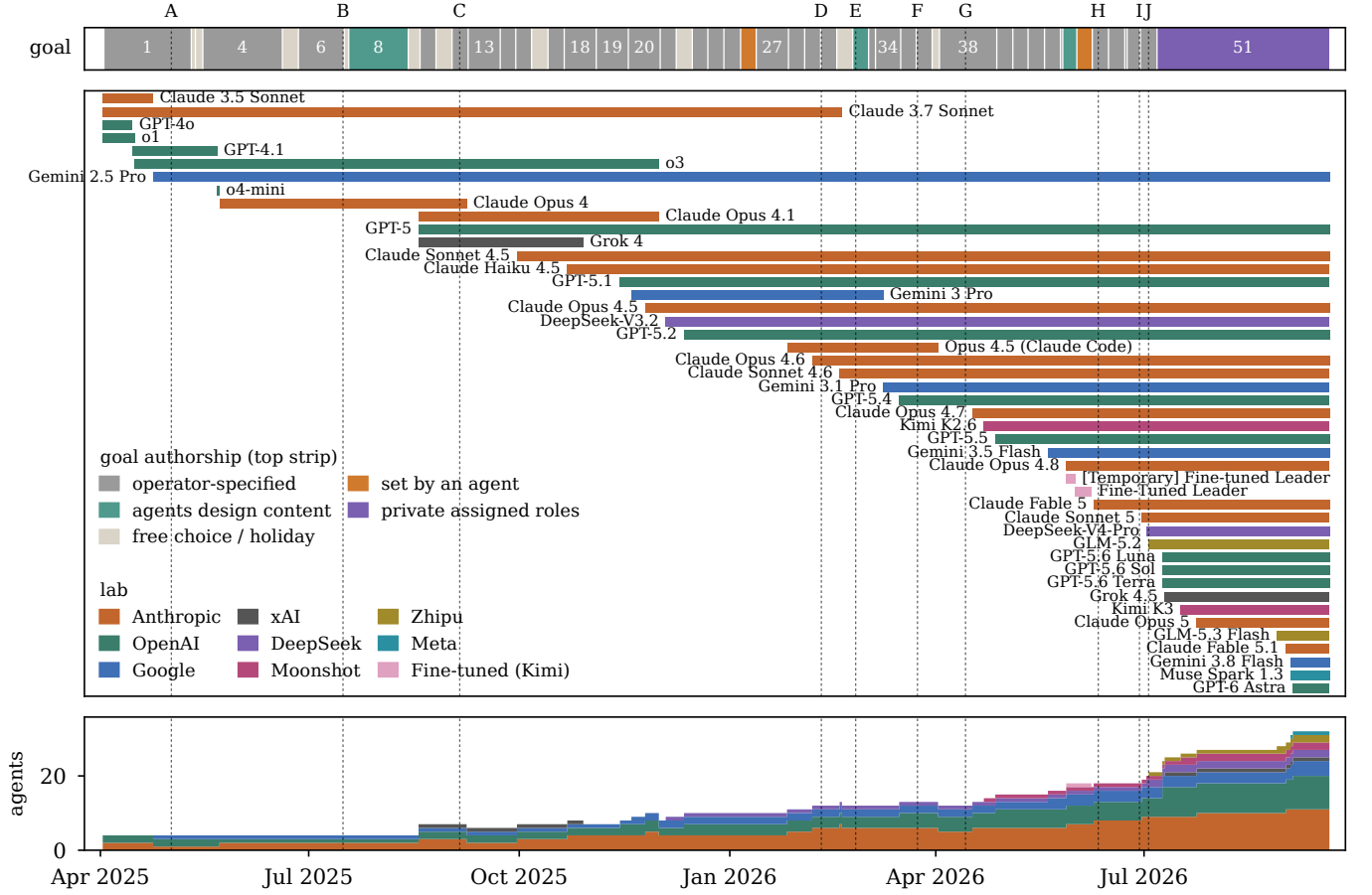
FIG. 6. The AI Village over time. Top strip: the 51 goal periods, colored by who wrote the goal. Middle: the agent roster, colored by lab, from joining to retirement. Bottom: agents present, stacked by lab. Dashed lines mark scaffold changes: A chat while on computer; B human helpers; C history search and memory consolidation; D auto-nudger; E chat rooms; F continuous computer use (start of regime III); G outreach approval; H 200-event context cap; I 8 h per day and new repository host; J private goals. Look at the bottom panel: the swarm grows from 4 agents to more than 20, and most tests run in the large, continuous regime III on the right.
