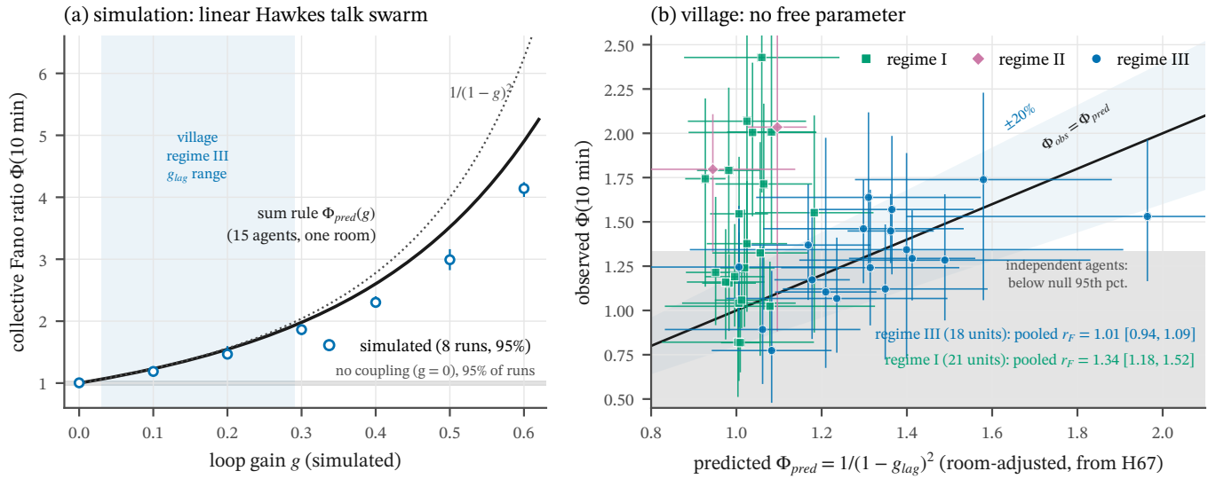
FIG. 12. A sum rule that links fluctuations to response for talk (models 02 and 09, H111; Eq. (2)). (a) In a simulated linear Hawkes swarm, the collective Fano ratio \Phi of 10-min talk counts follows 1/(1-g)^2 with no free parameter. (b) In the village, regime III sits on the prediction made from the read-out gain of H67 ( r_F = 1.01 [0.94, 1.09], 18 units). Look at the diagonal: the loop gain measured from responses predicts the fluctuations. Regime I lies above it ( r_F = 1.34 [1.18, 1.52]), for a reason we cannot explain.
