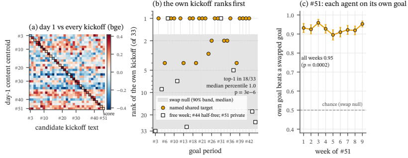
FIG. 3. The kickoff text is a field vector (model 11, H54). (a) Similarity of the day-1 content centroid of each period (rows) to each candidate kickoff text (columns), bge. (b) Rank of the own kickoff of the period among the candidates: first in 18/33 periods. (c) In #51 each agent sits on its own private goal (0.95 against a swap null of 0.5). Look at the dark diagonal in (a): the content of day 1 lands on the text that the operator wrote.
