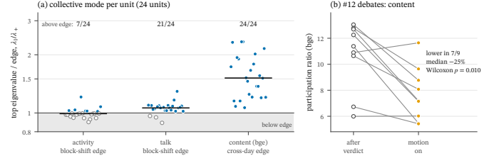
FIG. 5. Collective modes against a calibrated random-matrix edge (model 17, H12). (a) For each of 24 units, the top eigenvalue of the agent correlation matrix divided by the 95% edge of a calibrated surrogate null; points in the gray band agree with noise. Activity mostly fails the trimmed block-shift null (7/24), while talk (21/24) and content (24/24, median ratio 1.52) carry a real mode. (b) In the #12 debates, the participation ratio is lower while a motion is on than after the verdict in 7/9 debates (median -25%, p = 0.010 ). Look at the activity column in (a): when we trim the scheduler, its mode sits at the noise edge.
