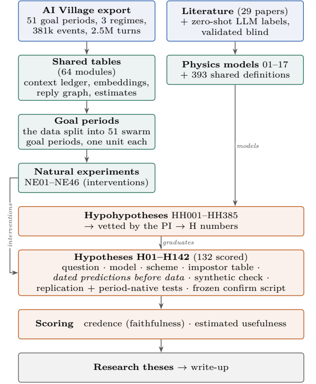
FIG. 7. The research loop. Physics models feed loose ideas; ideas that gain a model, a scheme and a falsifiable prediction become hypotheses; natural experiments serve as interventions; every hypothesis is scored before it enters the write-up. Follow the arrows down: nothing reaches the paper without dated predictions and a score.
