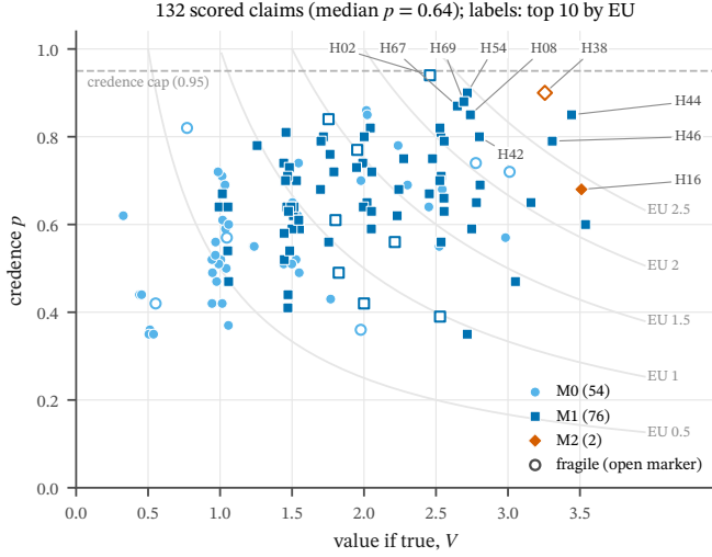
FIG. 10. Credence against value if true for every scored claim. Gray curves: equal estimated usefulness (EU). Marker: mechanism depth. Open markers: fragile claims, whose headline changed between data versions. Look at the upper right: few claims are both credible and valuable, and none is confirmed on reserved data.
