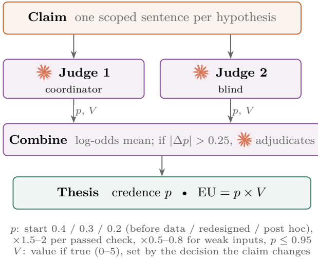
FIG. 8. Scoring. Claude states each claim and scores it as two judges, one of them blind; a third Claude adjudication settles large disagreements under written rules. The output is a credence p and an estimated usefulness EU = pV .
