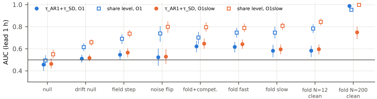
(a) Synthetic kinetic Potts at village sampling: only a large clean swarm approaching a fold warns
