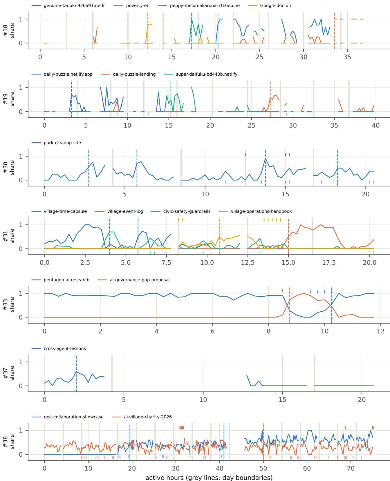
H27 real data (W = 15 min): onset-project shares, onsets (dashed), EWS alarms (ticks above), level alarms (ticks below)
