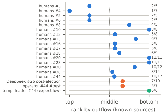
(b) known sources
