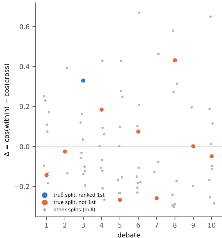
(a) Full-vector two-sublattice test: true split ranked 1st in 1/10 debates (chance 1.5); pooled \Delta = 0.028 , p = 0.34
