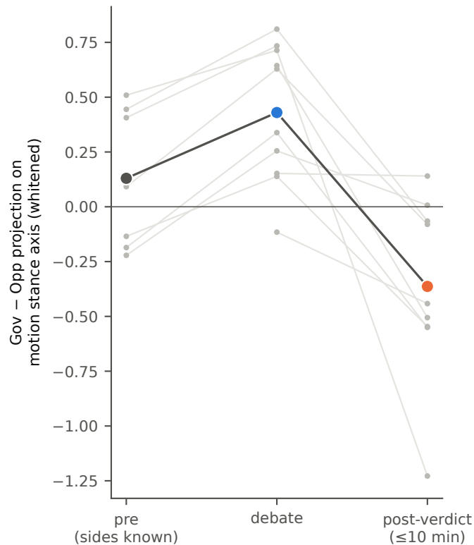
(b) Motion's a-priori stance axis: weak order in debate (9/10), flips after verdict (7/9)
