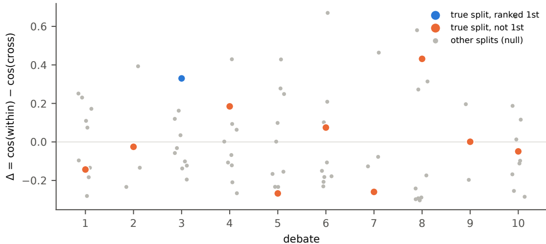
True split vs all other splits: recovered 1/10 (chance 1.5), p = 0.8
