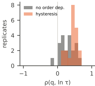
\tau_{\text{old}} (cosine)
