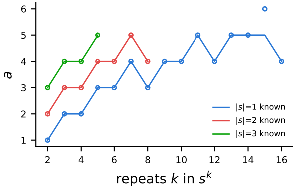
lines: |s| - 1 + \ell(k) ; circles: a_{RP}
