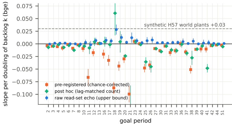
(b) within-agent echo slope vs backlog, per period
