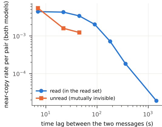
(a) near-copy rate by time lag, read vs unread pairs
