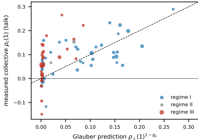
talk: collective memory beyond the prediction
