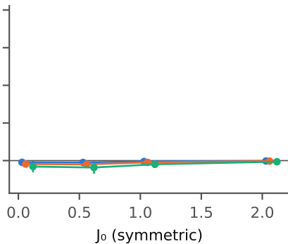
random order
