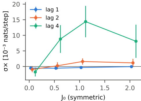
round robin
