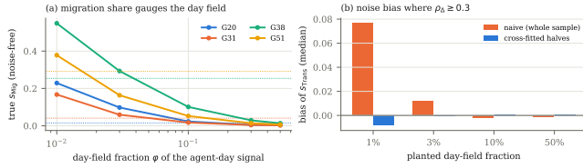
Second figure. Synthetic data at real counts. (a) The noise-free migration share falls steeply with the day-field fraction \phi . Dotted lines are the observed style shares. They imply \phi \approx 0.07 for style and 0.32 for content. (b) Without cross-fitting, sampling noise inflates transmission by up to 0.08. Cross-fitting removes this bias.
