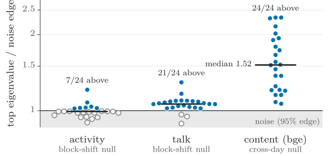
b #12 debates: content narrows while a motion is on
