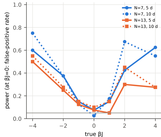
S4 plmDCA diagonal coupling (secondary)
