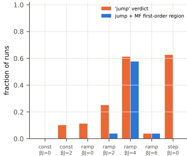
S3 jump detection (N=10, q=4, 5 d)
