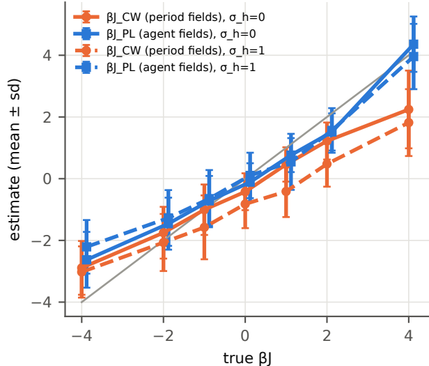
S2 confounds at \beta J = 0
