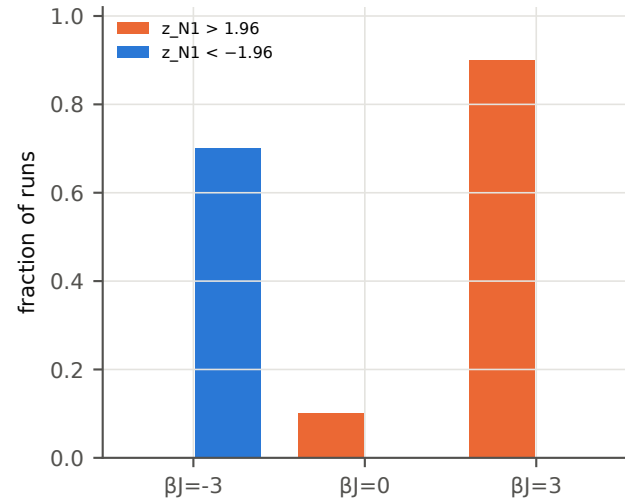
S4 plmDCA diagonal coupling (secondary)
