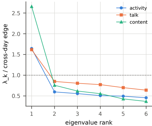
G19 spectra (19)
