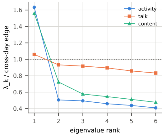
G40 spectra (40)
