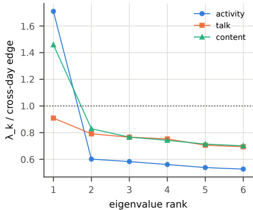
G42 spectra (42)
