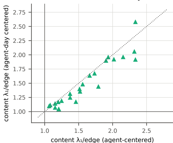
d Content mode survives day-centering
