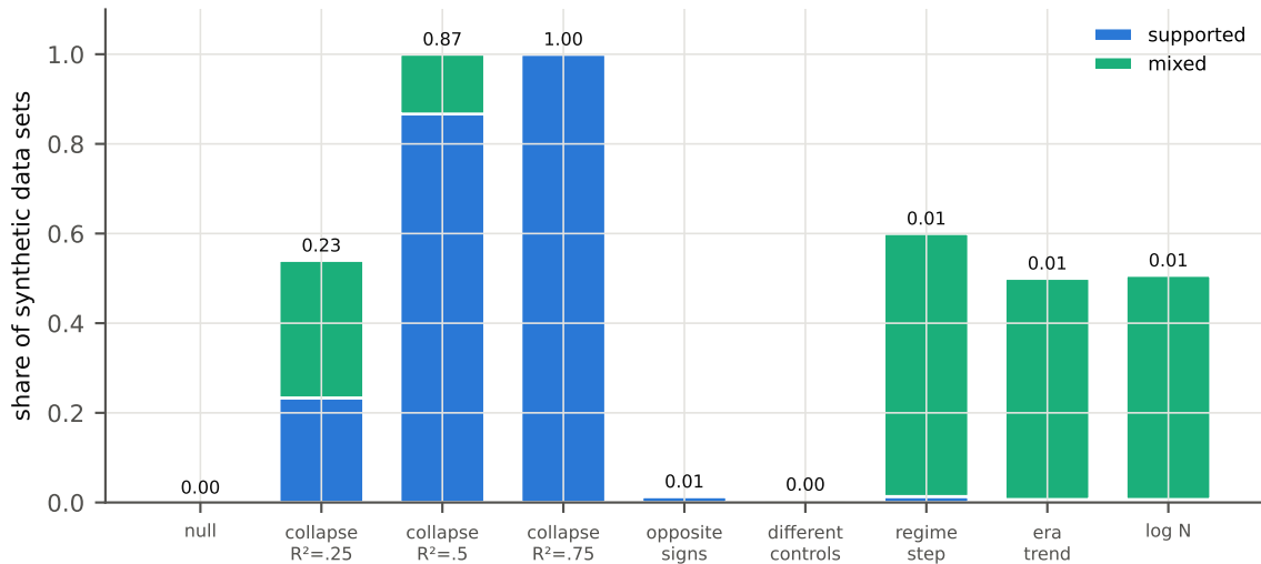
Synthetic validation (axis F): P1 verdicts on data simulated with the real design (periods, SEs, controls)
