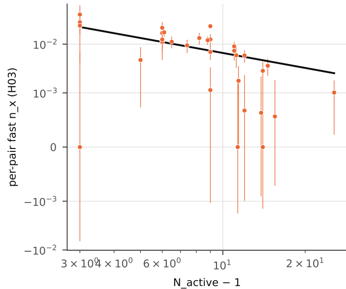
P4: exponent 1.02 [0.62, 1.43]
