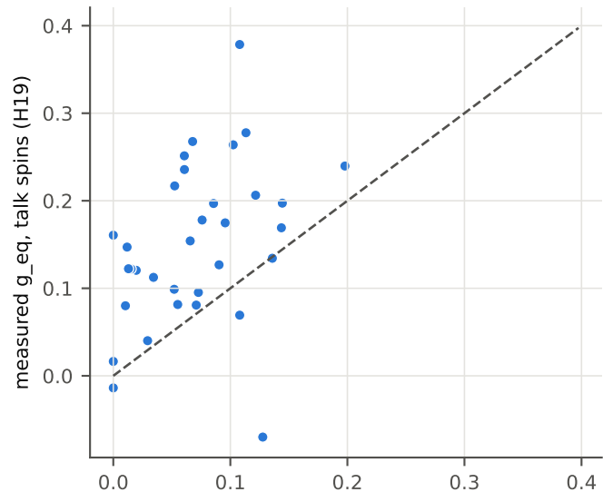
P3 mapping: \rho = +0.44 ; g_{eq} \geq \hat{g}_{map}(0.6) in 91%
