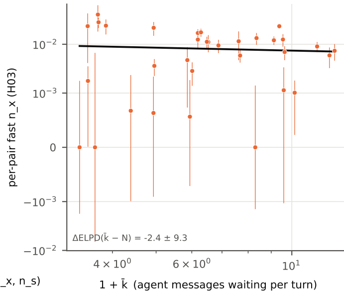
P4: exponent 0.20 [-0.61, 1.24]
