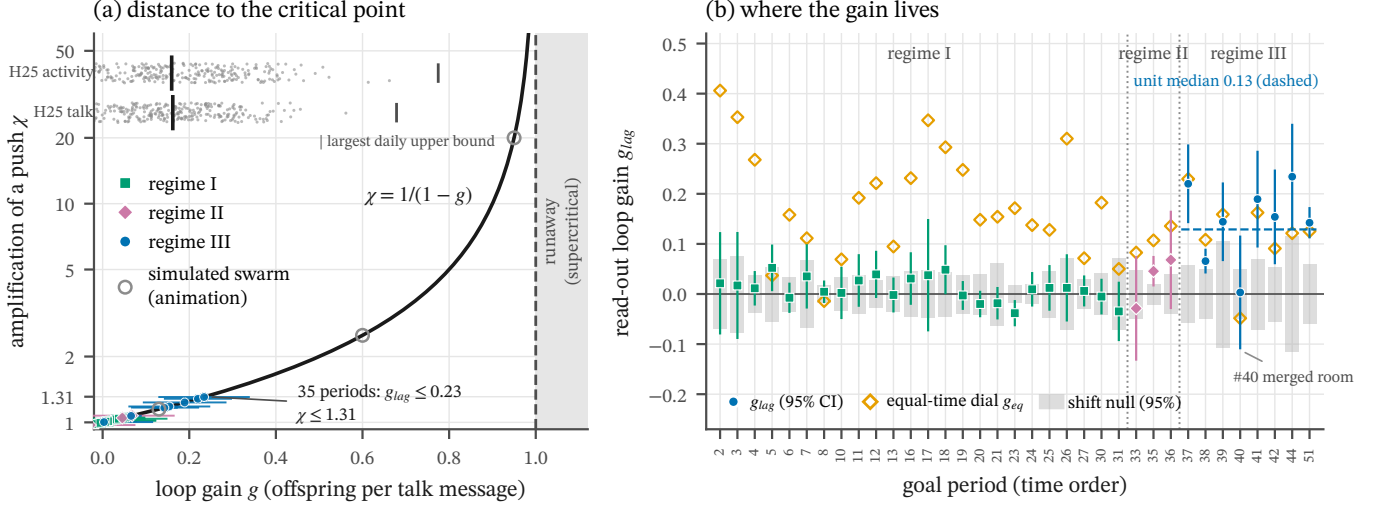
FIG. 6. The talk loop sits far below its critical point. (a) Amplification of a push, \chi = 1/(1 - g) , against loop gain g ; every goal period is placed at its read-out loop gain g_{lag} (H67, random-effects pool, 95% CI), and the gray strips are H25's daily equal-time Curie–Weiss dial for activity and talk (282 non-holdout days, medians 0.16; no day's upper bound reaches 0.8). The largest period gain is 0.23, so \chi \leq 1.31 , against a divergence at g = 1 ; open circles mark the simulated gains of the companion animation. (b) g_{lag} per period in time order: about 0 in regimes I and II, unit median 0.13 in regime III (every unit's upper bound < 0.40 ), with the shift null (gray, 95%) and the equal-time dial g_{eq} (orange), which reads 0.05–0.40 from fast shared fields where g_{lag} \approx 0 . Animation: H67-subcritical-dial/anim.mp4.
