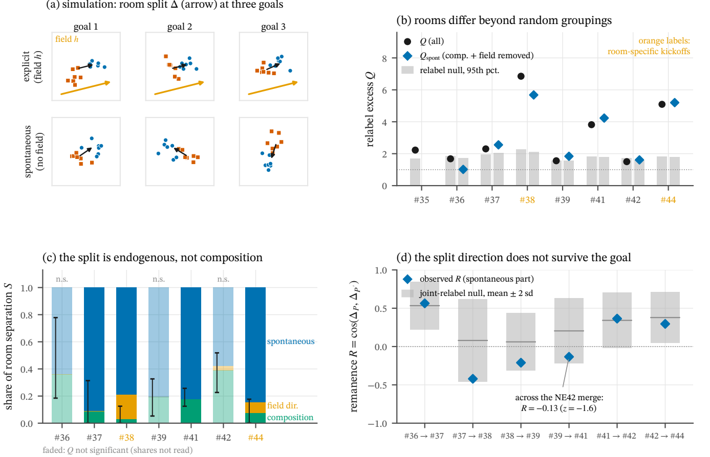
FIG. 19. The \#_{\text{best}}/\#_{\text{rest}} content split is spontaneous and regenerates at each goal (H100). (a) Simulation of a two-block soft-spin model: with a room field h the split \Delta points along h at every goal (explicit symmetry breaking); without one it takes a new direction at each goal (spontaneous). (b) Relabel excess Q of the split-half room separation per period, before and after removing composition and the measured field directions ( Q_{\text{spont}} ); gray: room-relabel null, 95th percentile. After both removals the rooms still differ beyond random groupings in 5/7 regime-III periods ( Q_{\text{spont}} 1.8–5.7). The two periods with room-specific kickoffs (orange) separate most ( Q 6.85, 5.09), but their split lies along the kickoff-text direction only at chance (#38: 0.18 vs null 0.16). (c) Shares of the separation: composition 0.03–0.18 where rooms separate significantly, spontaneous 0.58–0.91 (faded: Q not significant; bars: agent-bootstrap 95% CI of the composition share). (d) Remanence R of the spontaneous split direction between consecutive periods against the joint-relabel null (gray: mean \pm 2 sd): all six pairs have |z| < 2 , and across the NE42 merge R(\#39, \#41) = -0.13 ( z = -1.6 ). bge, style-residualized agent-day vectors. Animation: H100-room-symmetry-breaking/anim.mp4.
