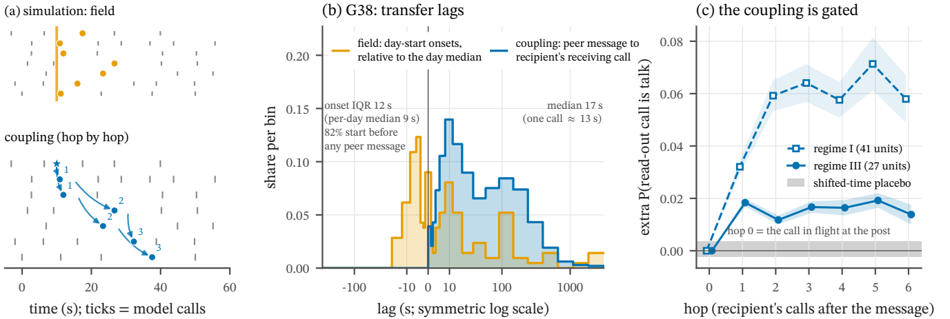
FIG. 2. Field or coupling: activity co-moves through the scheduler, talk spreads through one read-out call at a time. (a) Simulation on a synthetic call schedule (ticks: model calls, \sim 13 s apart). A field (orange line) reaches every agent at its next call, so all respond within about one call. A coupling passes from reader to reader, and each hop waits for the recipient's next call. (b) G38 (regime III), measured lags. Orange: each agent's first call of the day relative to that day's median (pooled IQR 12 s; per-day median IQR 9 s; 82% of agents start before any peer message reaches them). Blue: from a peer message to the recipient's receiving call (median 17 s; regime-III unit median 24 s). The tail is pauses. (c) Excess chance that a recipient's call is a talk call, by hop after a peer message (IVW pooled over 41 regime-I and 27 regime-III units; bands are 95% CIs). It is zero at the call in flight and steps up at the read-out call. The gray band is the pooled shifted-time placebo. J_1 > 0 in 45/71 units and < 0 in none. The regime-I rise beyond hop 2 is not validated on synthetic data. Animation: H50-field-vs-coupling-transfer-lag/anim.mp4.
