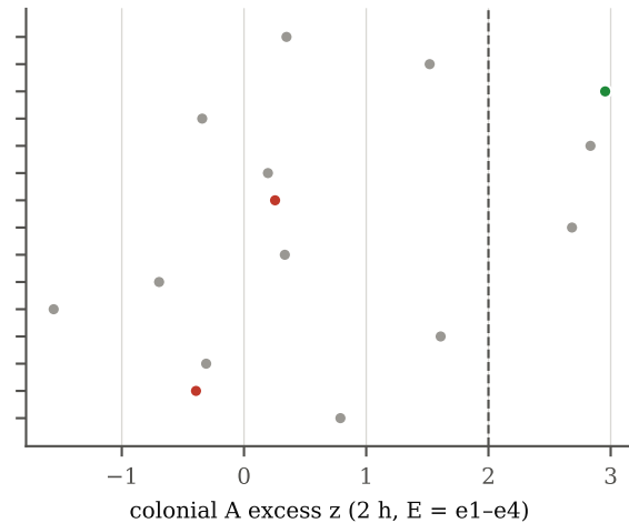
P3a (green: P2 + z \geq 2 ; red: P2, z < 2 )
