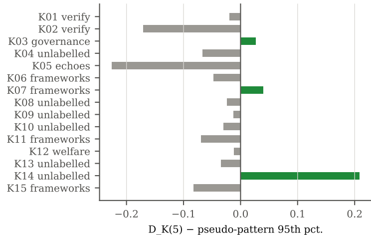
P2: host renewal (green = pass)
