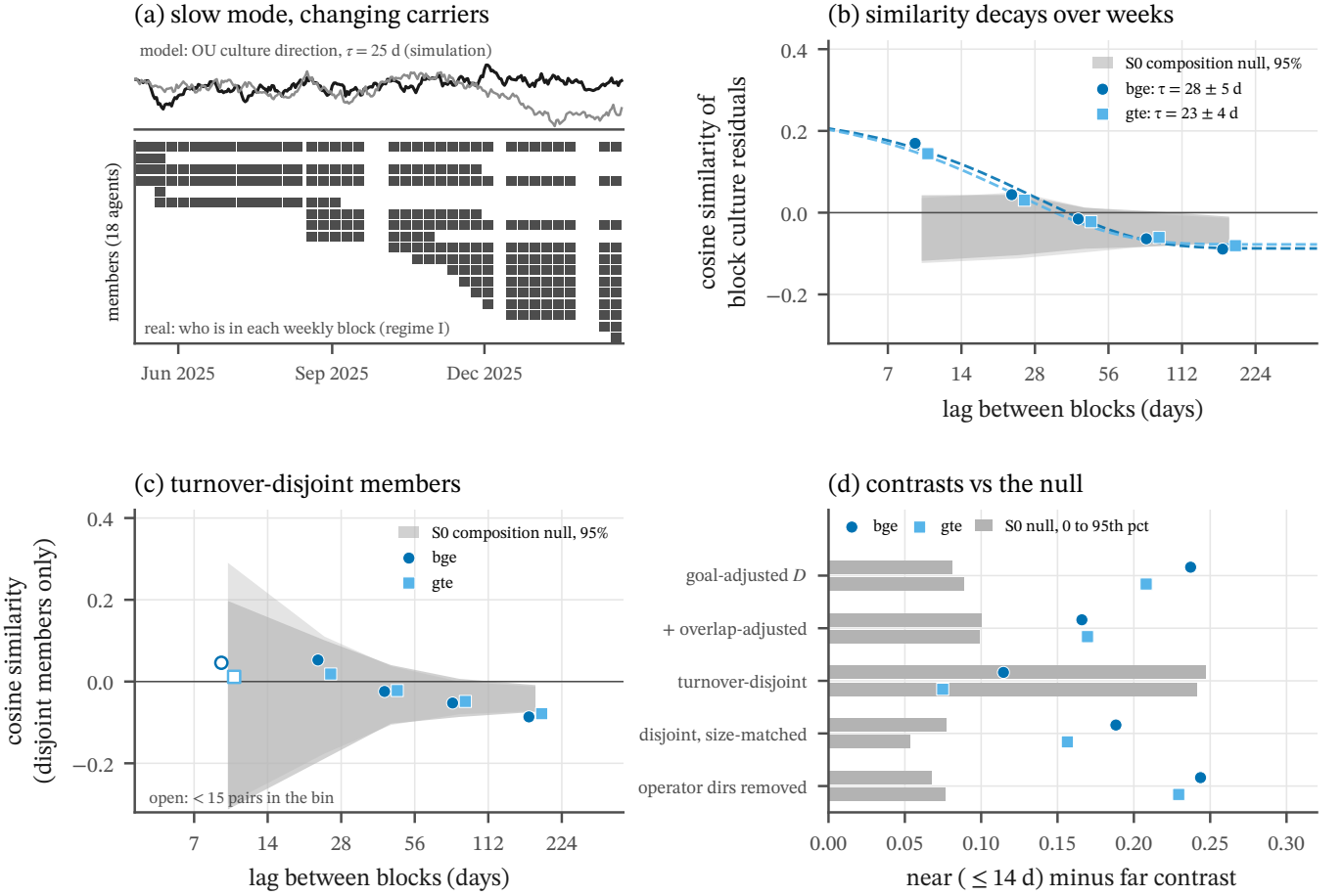
FIG. 11. Regime-I content has a slow collective mode beyond its members and the measured fields (H81). (a) The Ornstein-Uhlenbeck model and the weekly roster of regime I. (b) Similarity of block culture residuals against lag for two embedding models, with the 95% band of the S0 composition null and OU fits \tau_u = 28 \pm 5 and 23 \pm 4 d. (c) The turnover-disjoint profile. (d) The near-minus-far contrasts against their null 95th percentiles.
