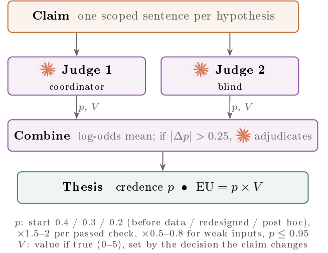
FIG. 3. Scoring. Claude states each claim and acts as two judges, one of them blind. A third Claude adjudication settles large disagreements under written rules.
