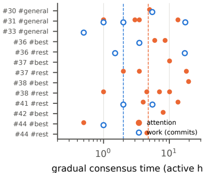
b Attention vs work
