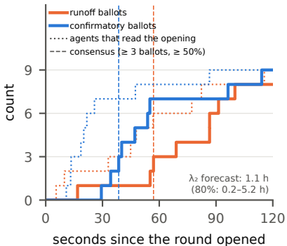
a #26 votes: read-out speed
