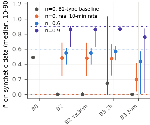
synthetic guard (TALK+ALL)
