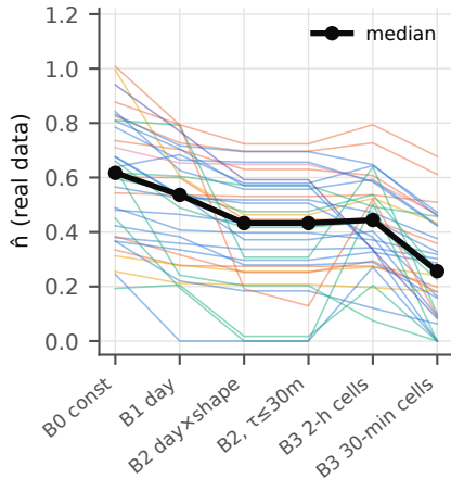
ALL: baseline ladder
