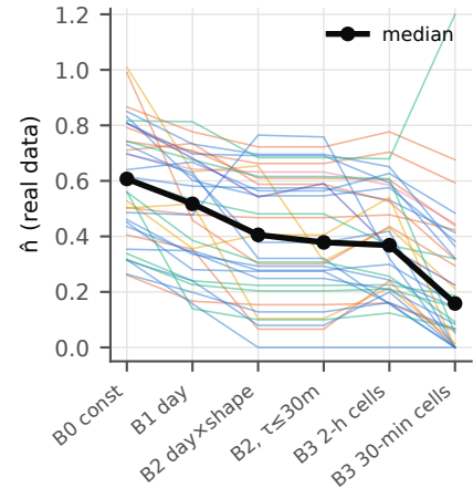
TALK: baseline ladder
