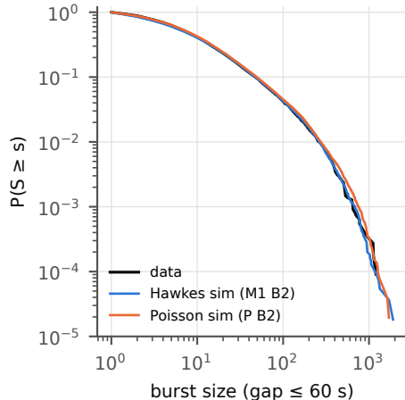
ALL: bursts (pooled periods)
