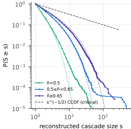
TALK: cascades (dots: Borel( \hat{n} ))
