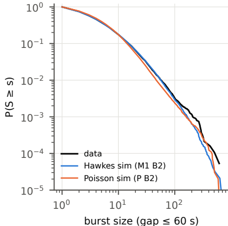
TALK: bursts (pooled periods)
