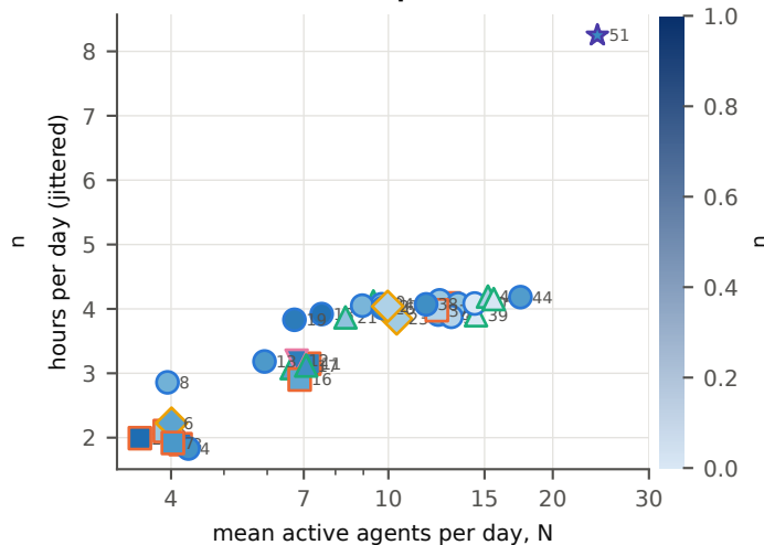
ALL: N × hours plane, fill = \hat{n}
