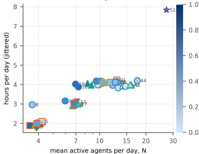
TALK: N × hours plane, fill = \hat{n}
