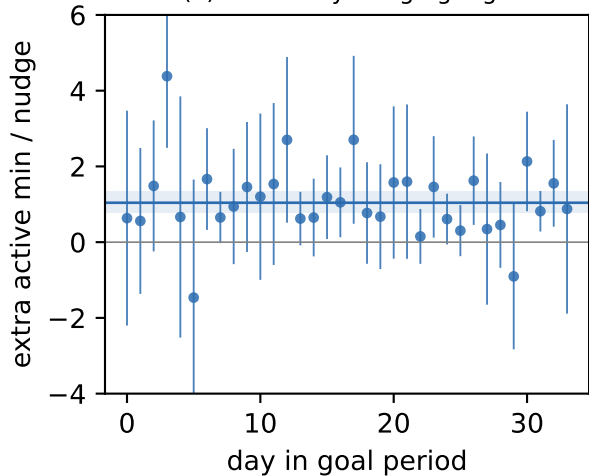
(a) G51: daily nudge gauge
