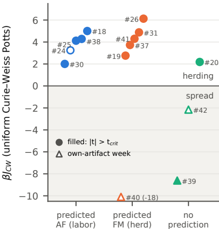
a Herding whatever the mode
