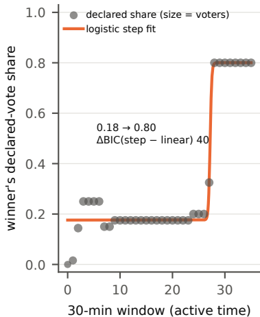
b #26 runoff jump
