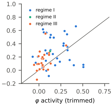
(b) shared share \phi
