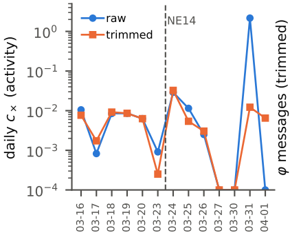
(a) regime II \rightarrow III
