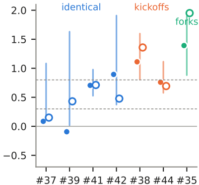
onset ratio r_1 = E(1)/E_F
