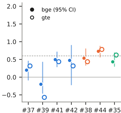
onset projection \pi_1
