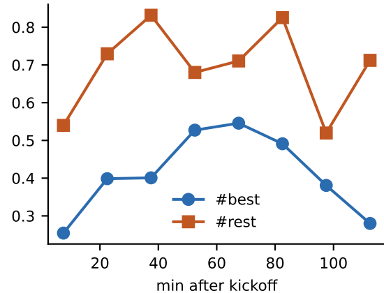
kickoff #37: L -0.28 (p 0.18)
