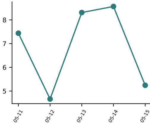
between-room separation F per day
