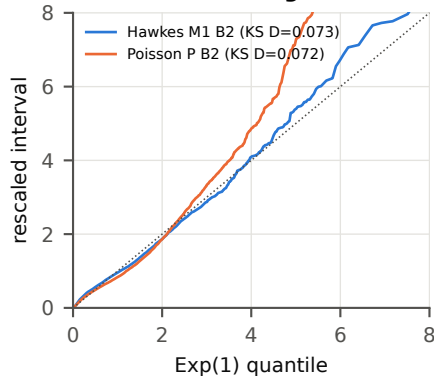
(b) time-rescaling QQ, TALK
