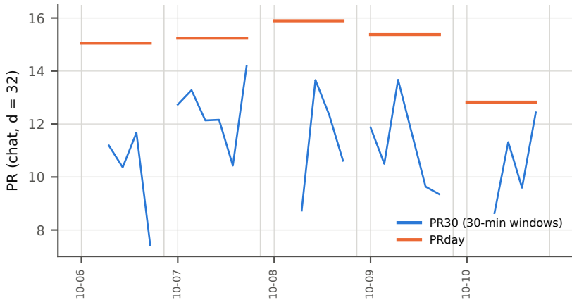
dimensionality by window and day
