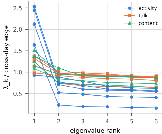
G51 spectra (51a, 51b, 51c, 51d, 51e)
