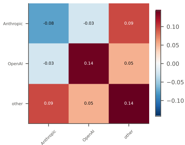
content co-movement: K \times K mean-field J ; \Delta = -0.047 ( p = 0.61 )
