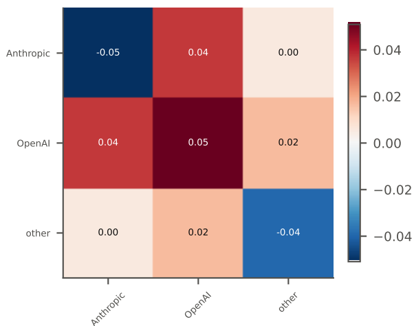
talk spins: K \times K mean-field J ; \Delta = -0.035 ( p = 0.72 )
