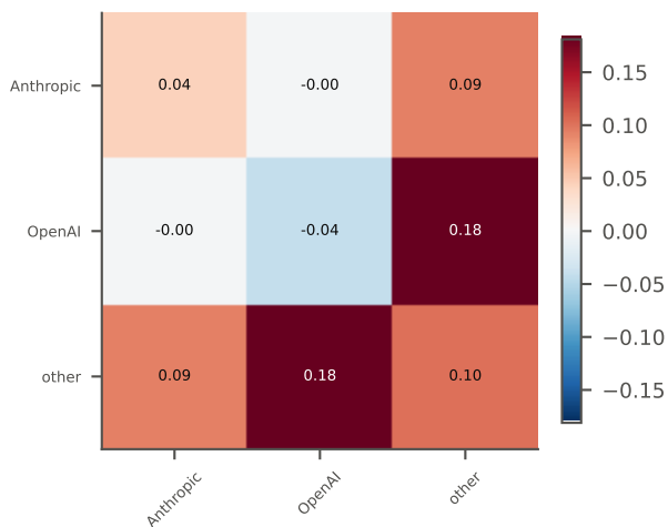
talk spins: K \times K mean-field J ; \Delta = -0.041 ( p = 0.56 )
