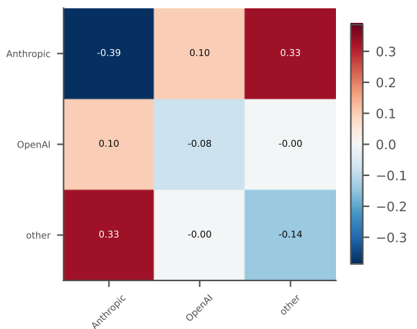
talk spins: K \times K mean-field J ; \Delta = -0.486 ( p = 0.99 )
