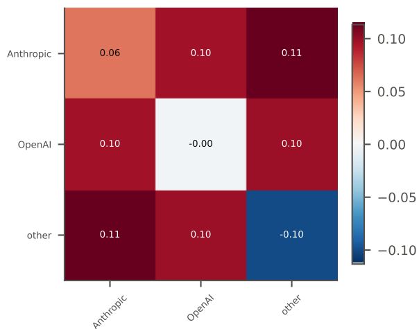
content co-movement: K \times K mean-field J ; \Delta = -0.060 ( p = 0.58 )
