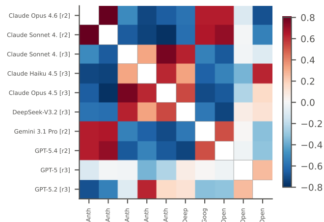
unit 38b: \cos(H_i, H_j) , lab order; T = -0.03 ( p = 0.455 )
