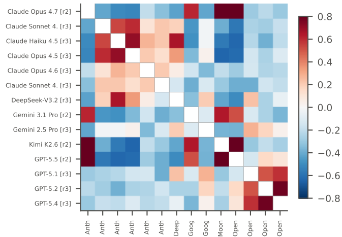
unit 41: \cos(H_i, H_j) , lab order; T = 0.28 ( p = 0.011 )
