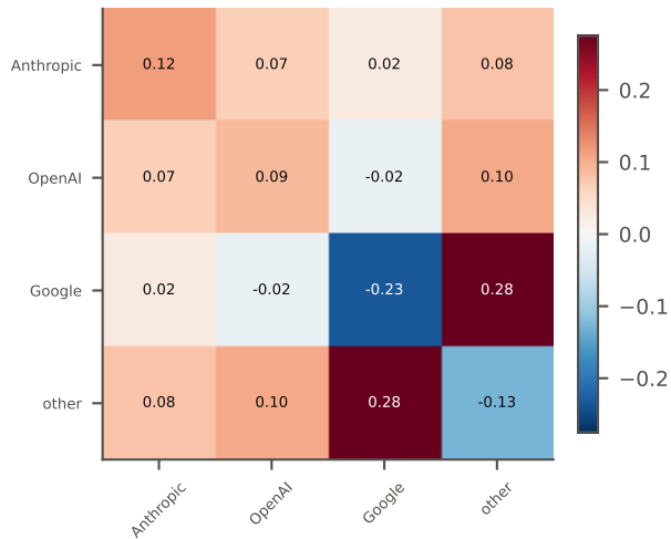
content co-movement: K \times K mean-field J ; \Delta = 0.032 ( p = 0.07 )
