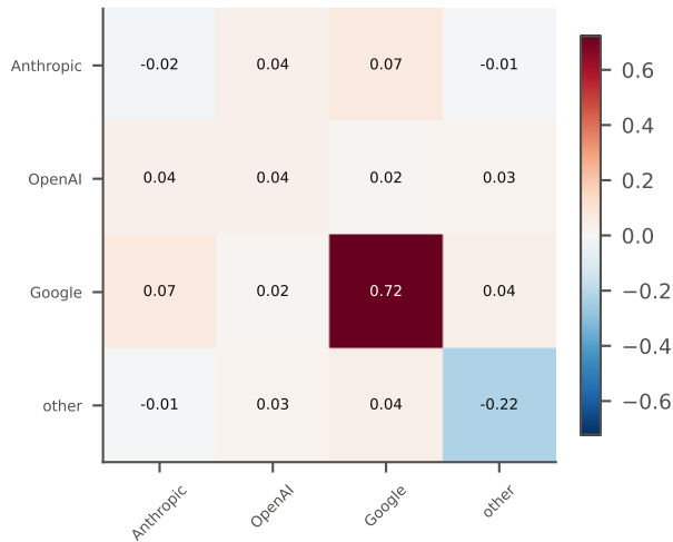
talk spins: K \times K mean-field J ; \Delta = 0.002 ( p = 0.41 )
