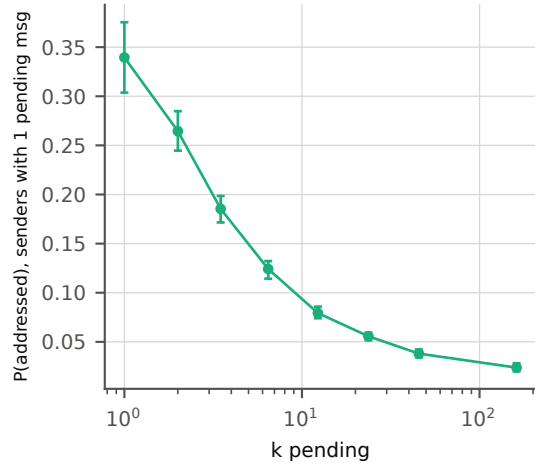
G51: \hat{\beta} = 0.61 [0.58, 0.63]
