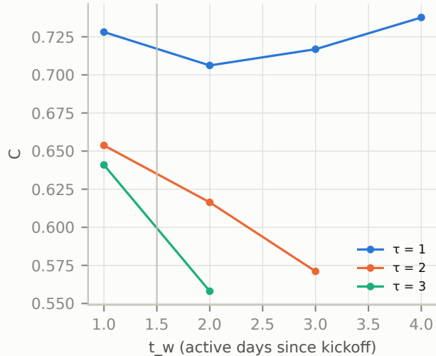
A = +0.006 ( p = 0.443 ); A_late = +0.072
