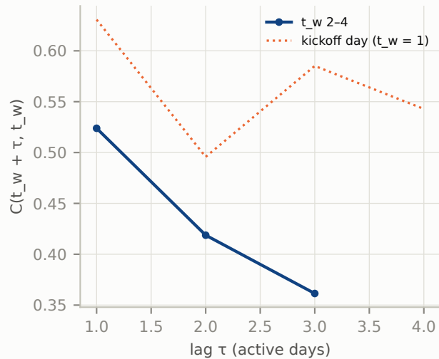
#35: C by age band
