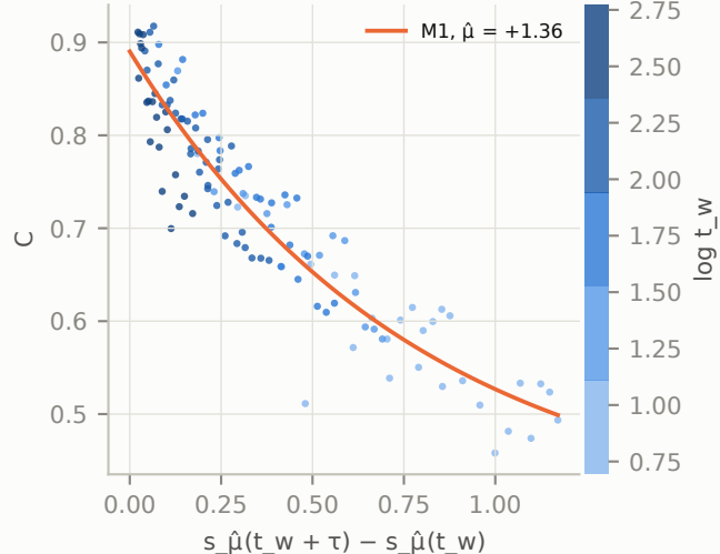
collapse, \hat{\mu} CI [ +0.86 , +1.84 ]
