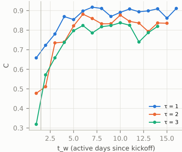
A = +0.102 ( p = 0.002 ); A_{\text{late}} = -0.043
