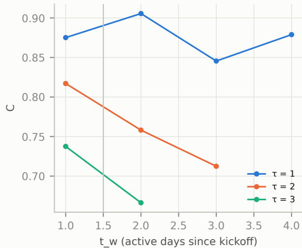
A = -0.061 ( p = 0.749 ); A_{\text{late}} = +0.116
