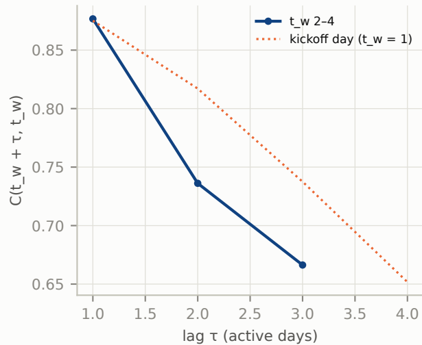
#40: C by age band
