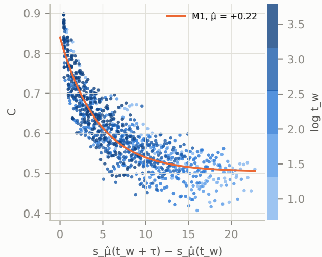
collapse, \hat{\mu} CI [ +0.07 , +0.41 ]
