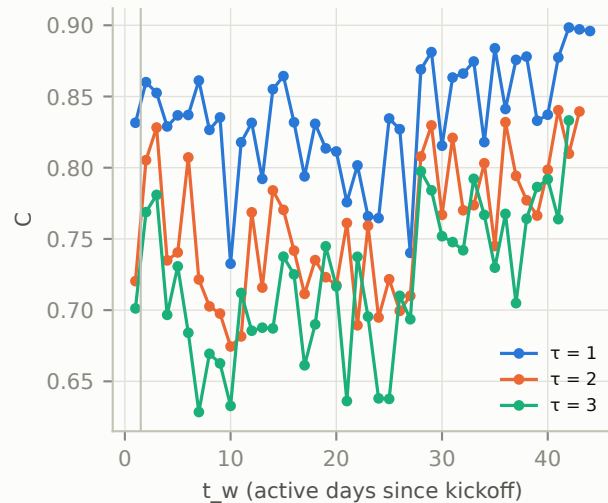
A = +0.012 ( p = 0.078 ); A_{\text{late}} = +0.111
