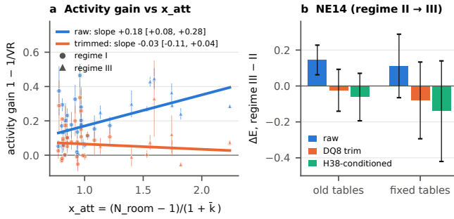
Second figure. (a) Activity gain per period vs x_{att} , raw (blue) and day-edge-trimmed (orange), with meta-regression lines. The rise disappears after the trim. (b) NE14: the regime II→III change of the activity gain, raw vs trimmed vs H38-conditioned, on old and fixed tables.
