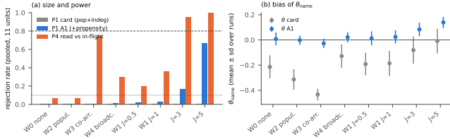
Second figure. Synthetic validation on 11 real skeletons (G38, G31, 51c, 51h; 60–300 runs per world). (a) Rejection rates. The card’s P1 never rejects, because its \theta_{\text{name}} is biased negative. A1 has size \leq 0.013 but power 0.02 at J = 1 and 0.67 only at J = 5 . P4 has power 0.36 at J = 1 , but co-arrival (W3) fakes it in 74% of runs. (b) Bias: with no following (W0) the card’s \theta_{\text{name}} is -0.21 \pm 0.09 , because namers hop more; A1 removes the bias.
