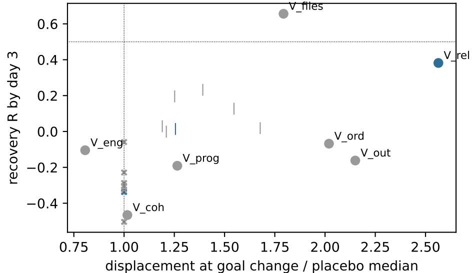
regime III: 5 goal-change shocks; chosen V_{rel} (inconclusive)
