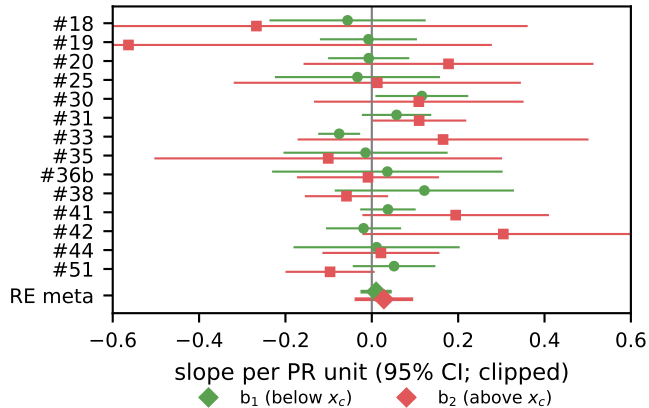
(b) per period at x_c (14 of 17 estimable)
