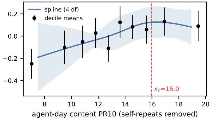
(a) pooled, 1592 agent-days, 17 periods b_1 = +0.035 (p 0.26), b_2 = -0.035 (p 0.35)
